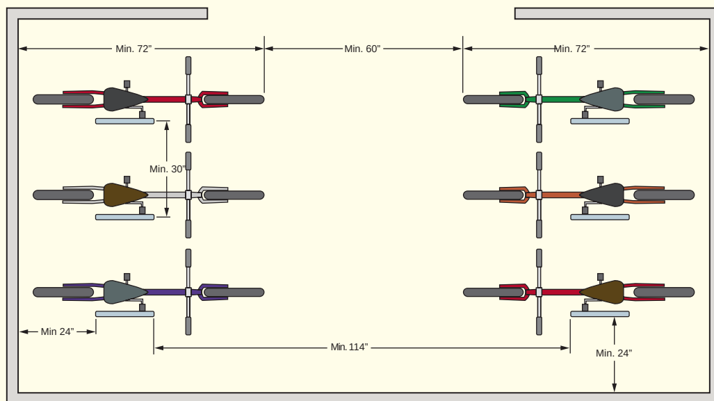
Diagram 3: Bicycle Parking Location and Design (top view).
