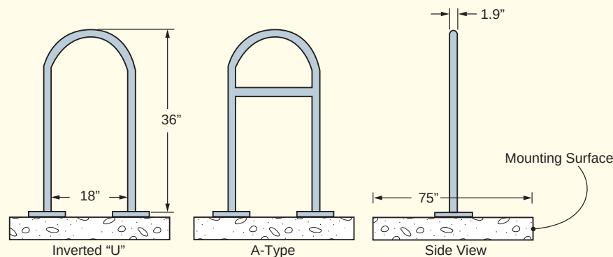
Diagram 2: Bicycle Parking Location and Design (side view)
